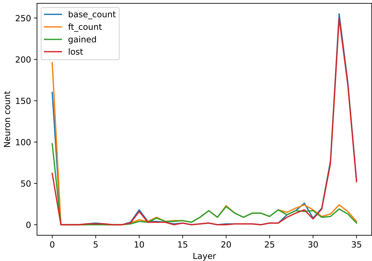
hi (src): counts (base vs ft)
