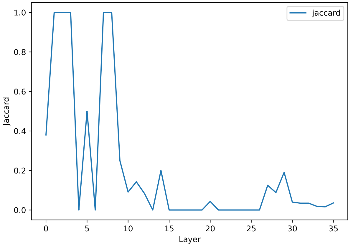
hi (src): per-layer Jaccard (base vs ft)
