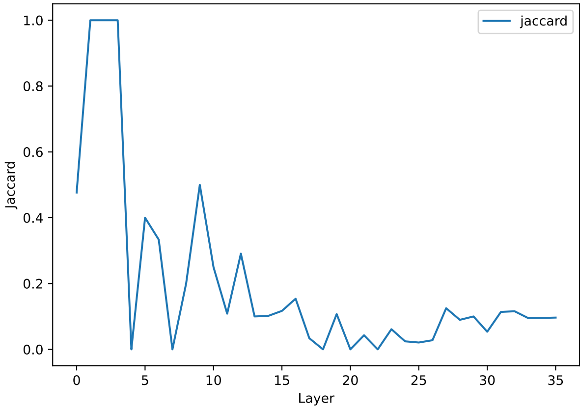
te (src): per-layer Jaccard (base vs ft)
