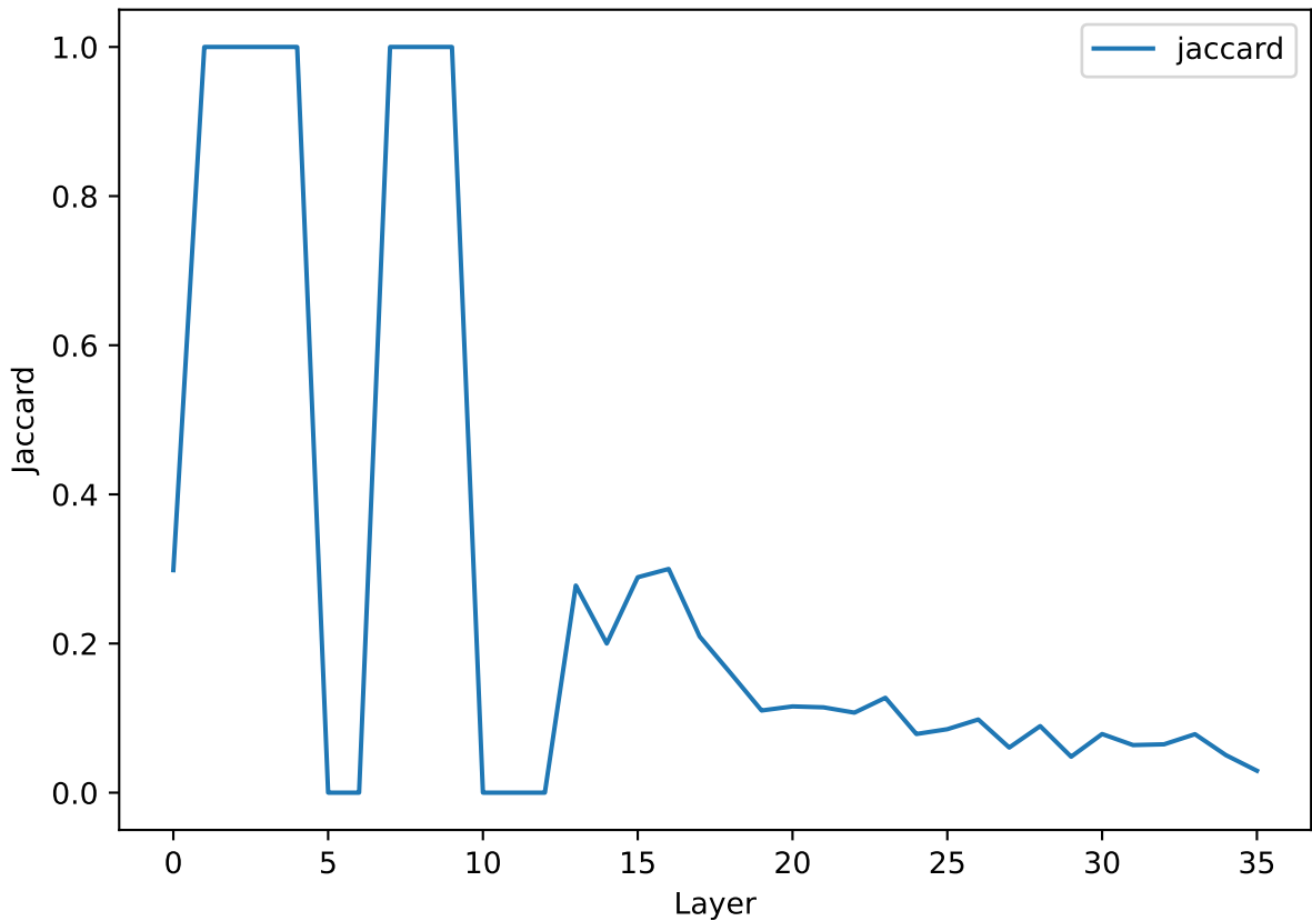
bn (tgt): per-layer Jaccard (base vs ft)
