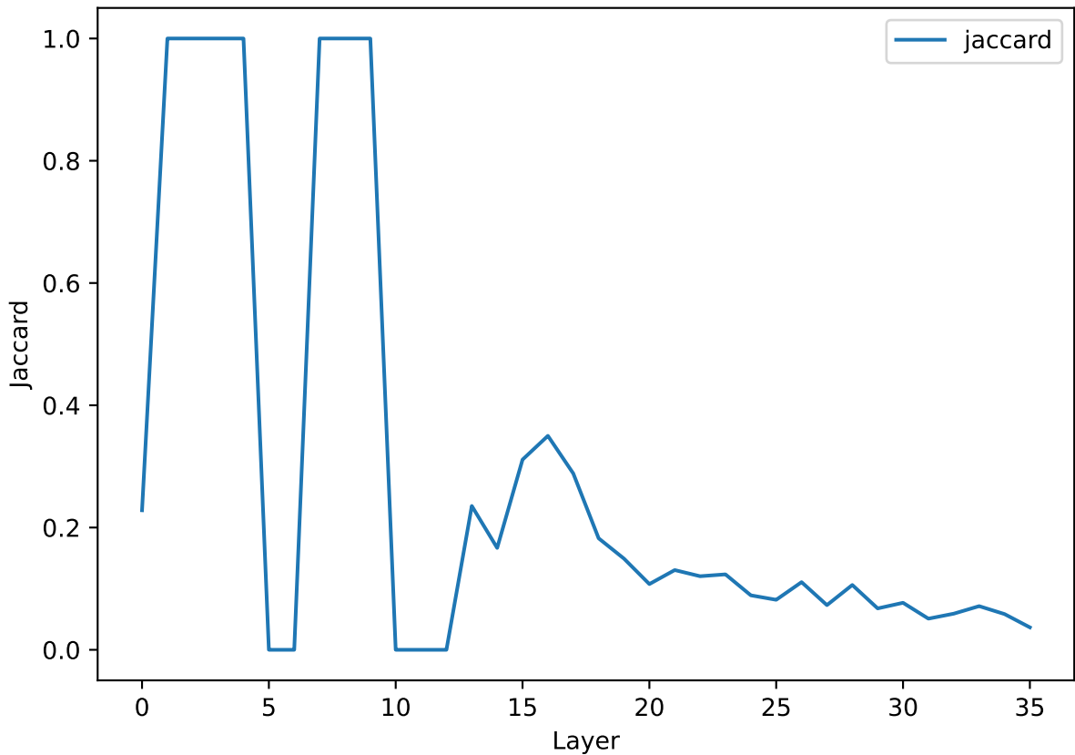
hi (tgt): per-layer Jaccard (base vs ft)
