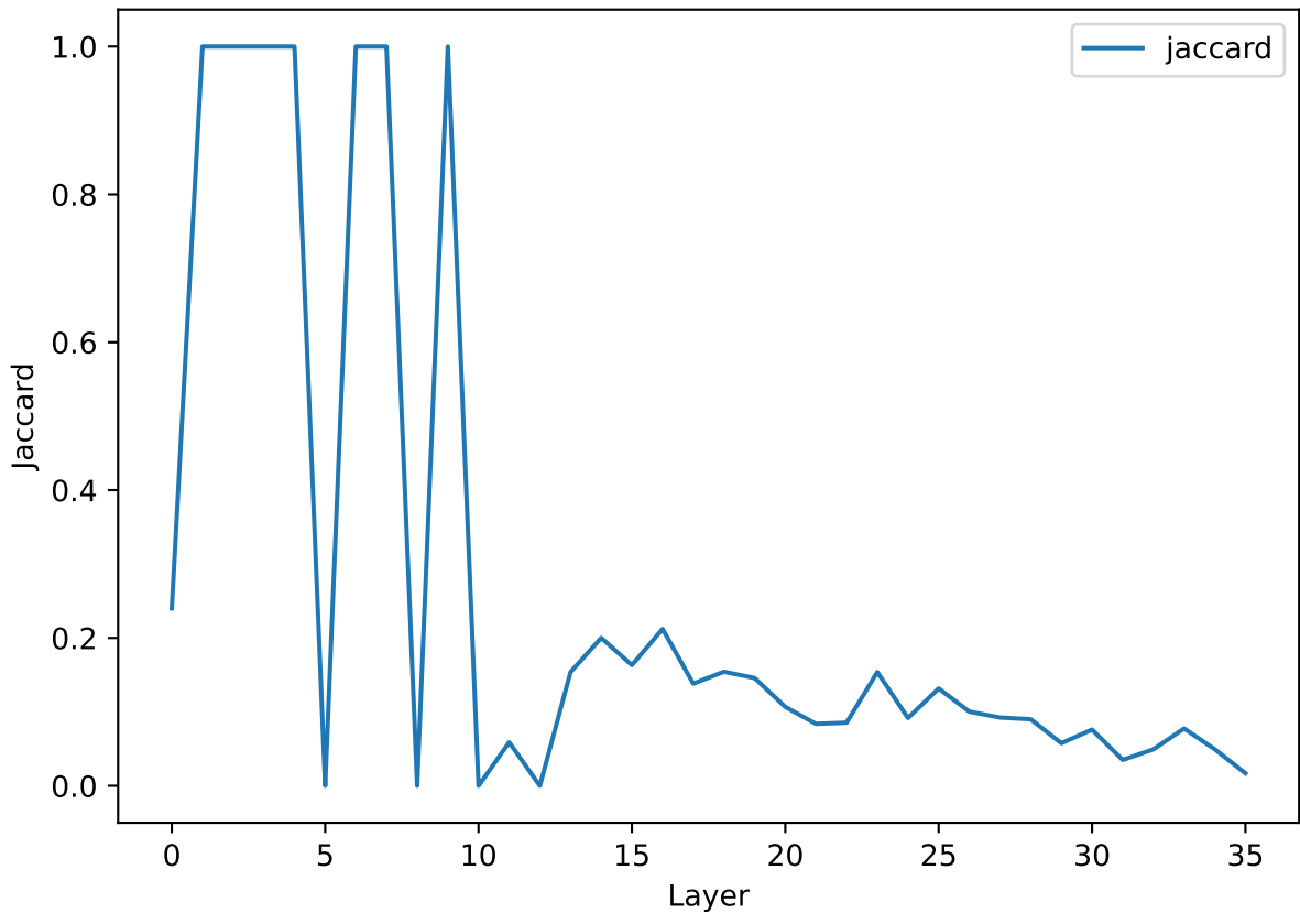
te (tgt): per-layer Jaccard (base vs ft)
