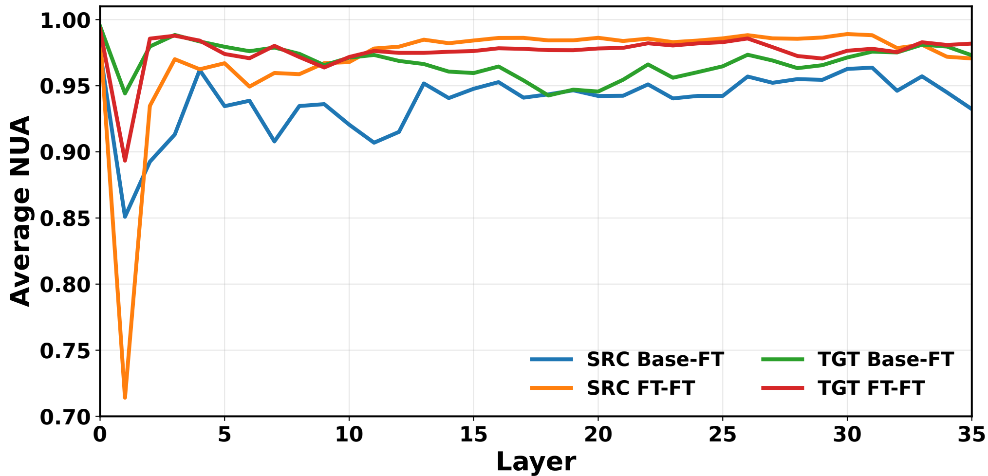
En->XX: Average Base-FT vs FT-FT Neuron Usage Alignment
