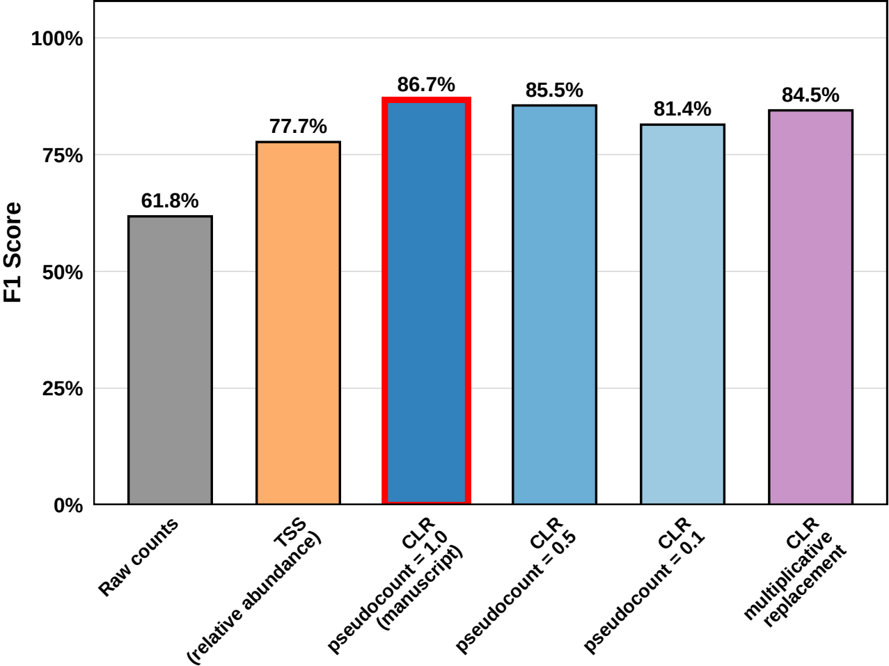
Test Set F1 Score by Normalization / Zero-Handling Strategy
