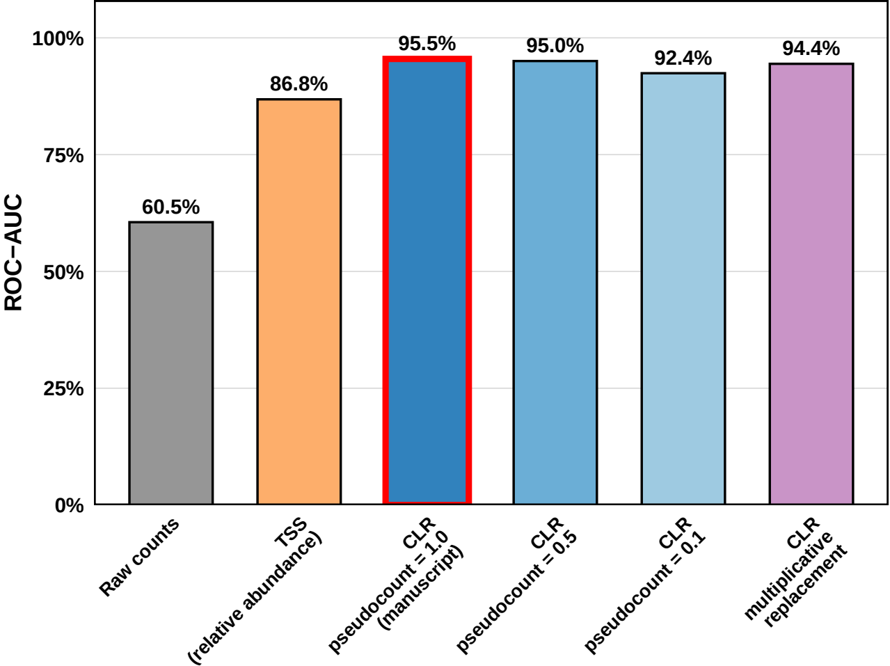
Test Set ROC-AUC by Normalization / Zero-Handling Strategy
