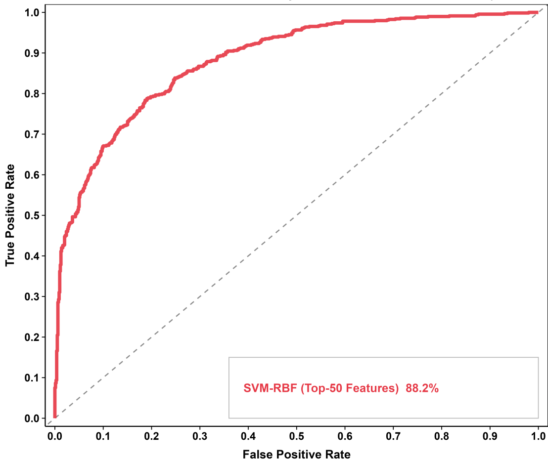
ROC Curve of SVM-RBF Trained on Top-50 Features on Test Dataset (n = 1,491)
