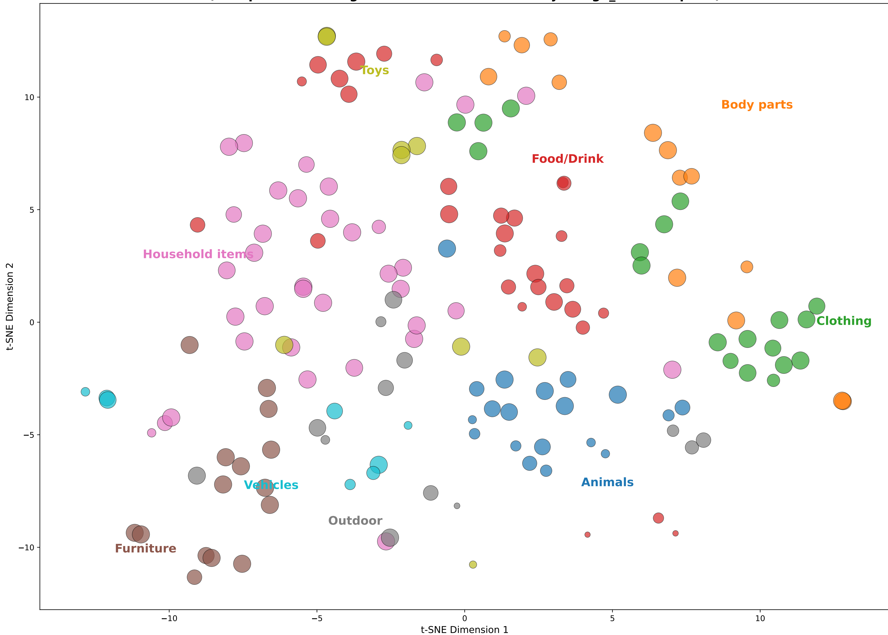
t-SNE Visualization of Object Classes by CDI Categories (Grouped embeddings: dot size = number of subject/age_mo exemplars)
