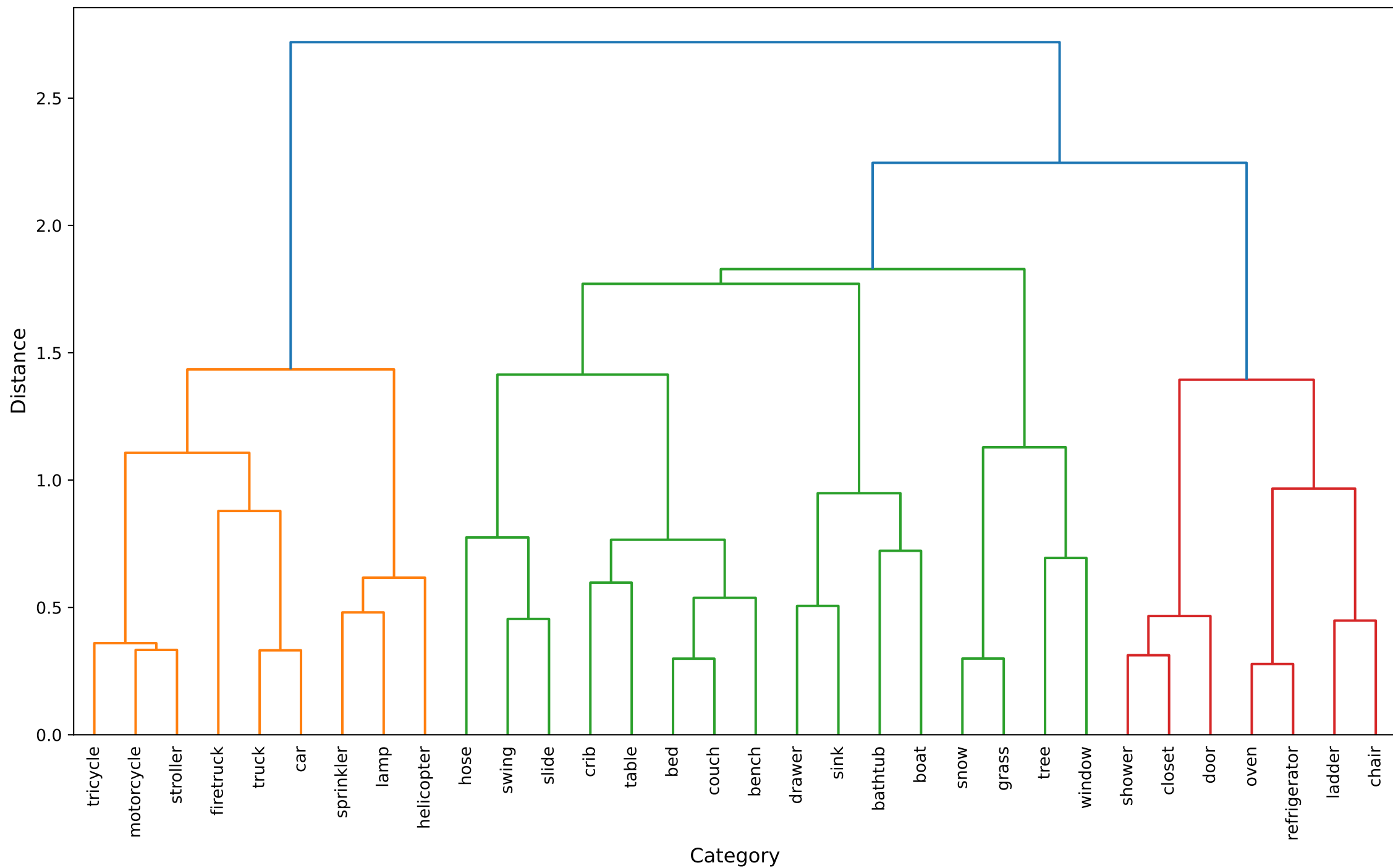
Hierarchical Clustering Dendrogram: BIG_OBJECTS\n(32 categories)
