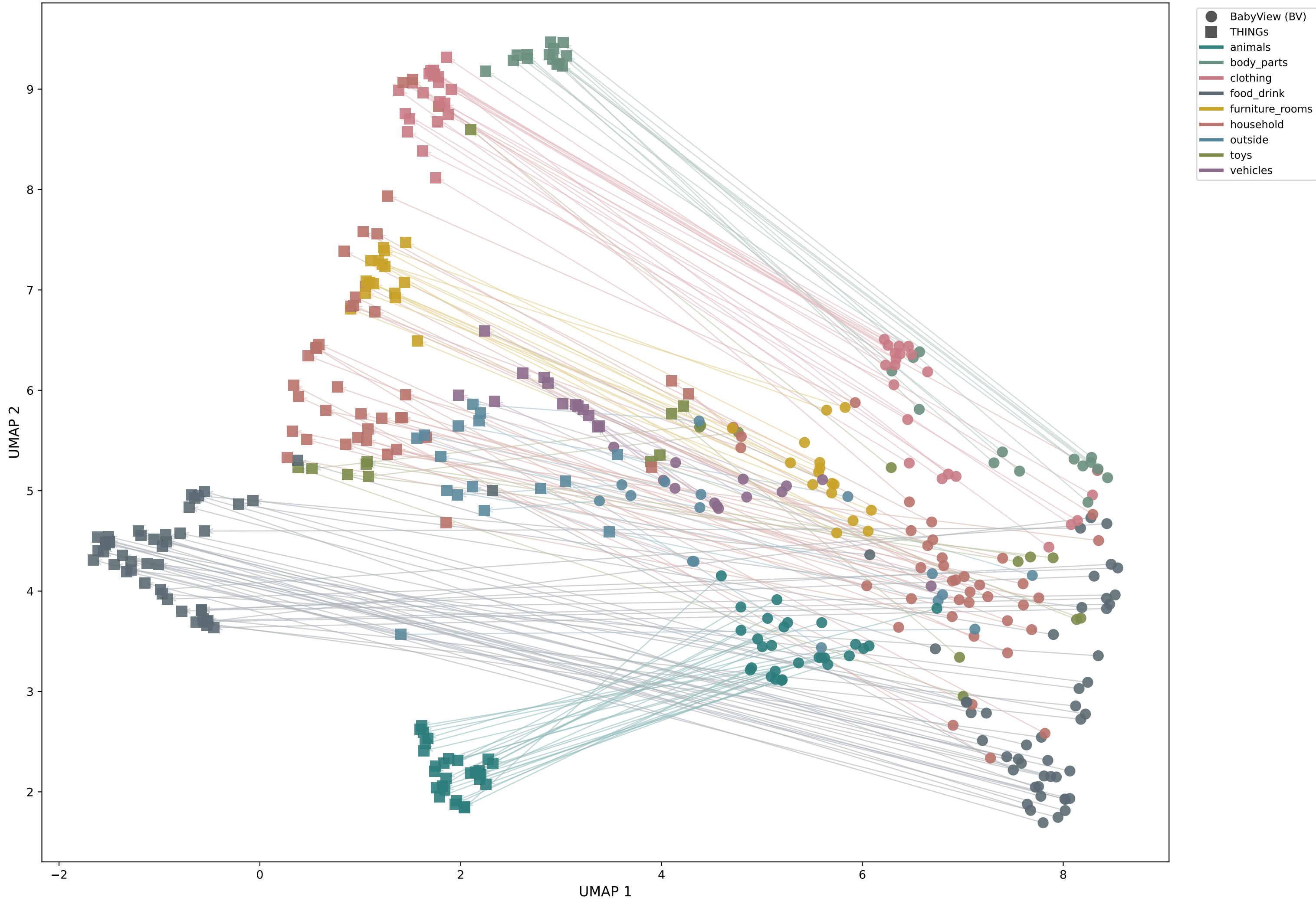
UMAP: BabyView vs THINGs category embeddings (Line connects BV → THINGs for each category)
