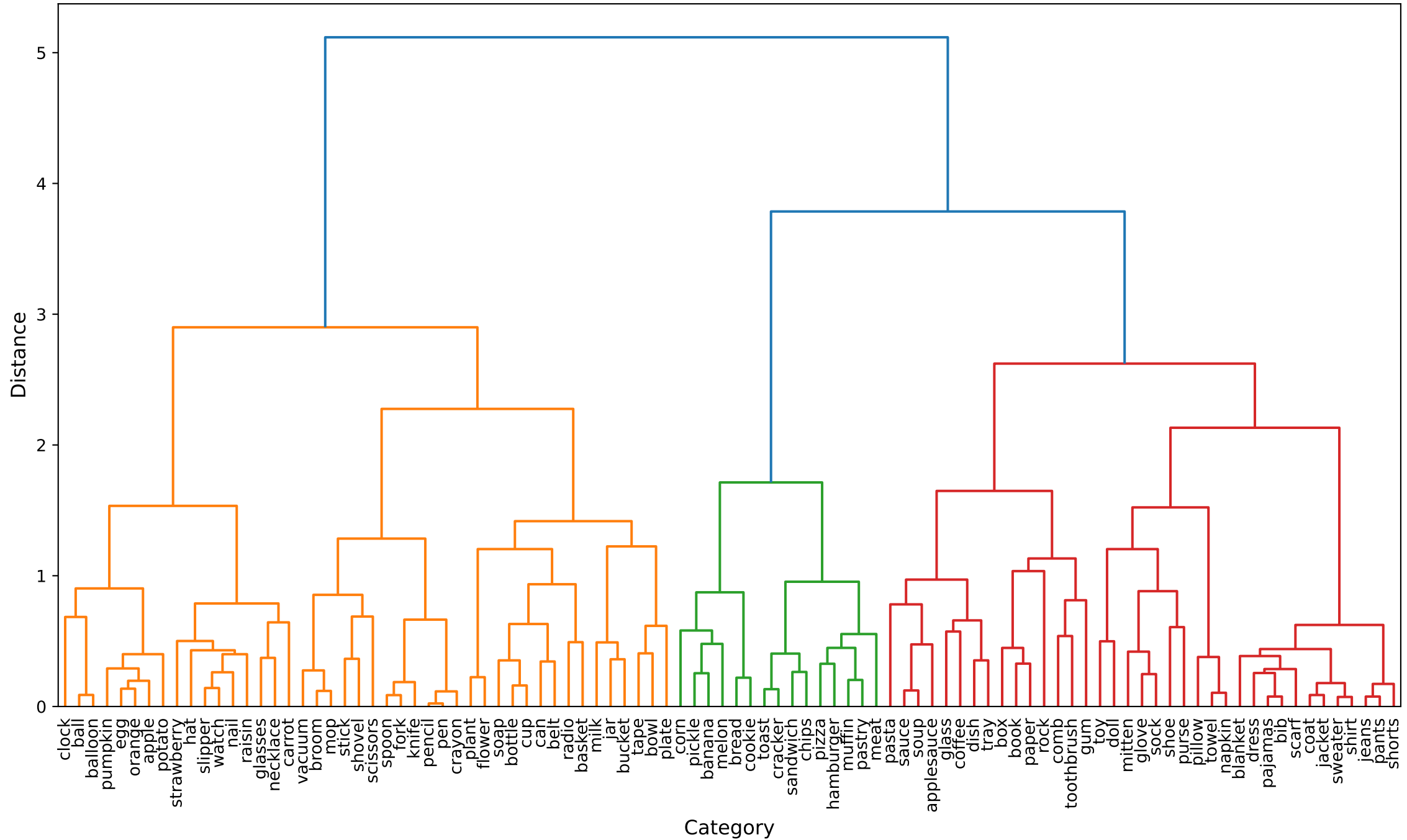
Hierarchical Clustering Dendrogram: SMALL_OBJECTS (96 categories)
