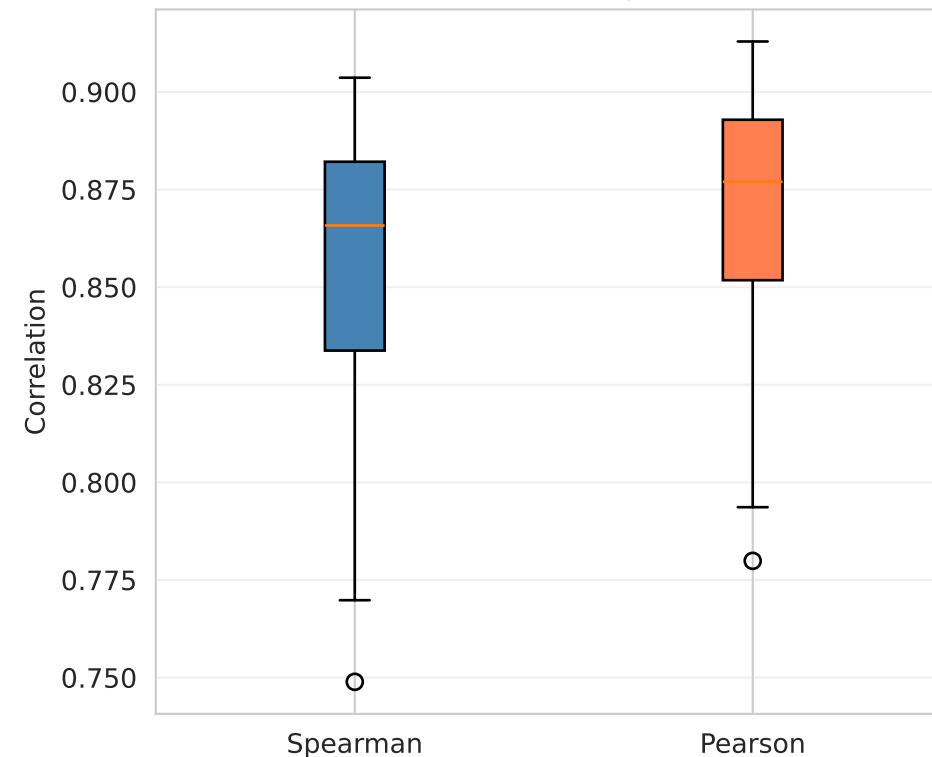
Correlation Comparison
