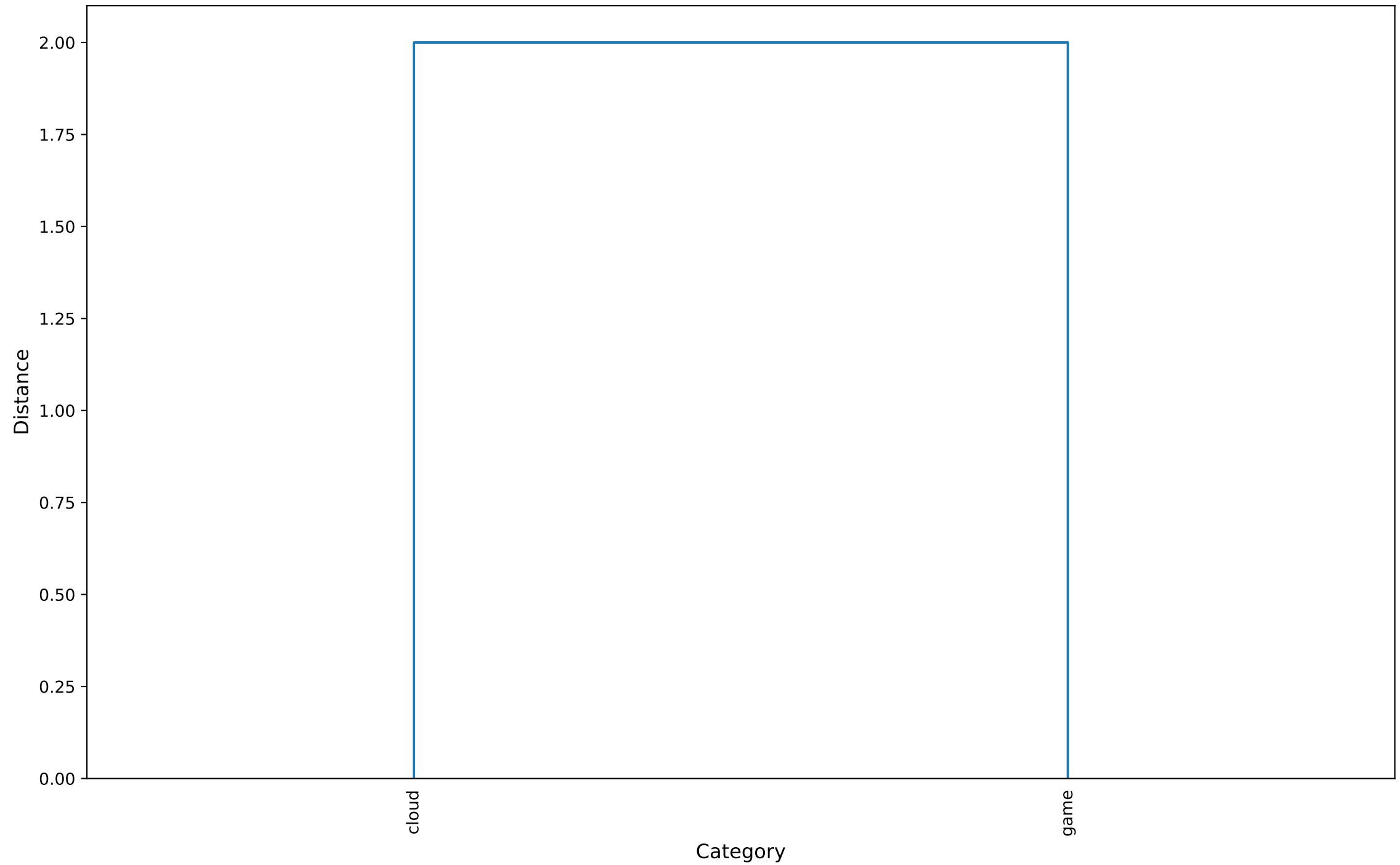
Hierarchical Clustering Dendrogram: OTHERS\n(2 categories)
