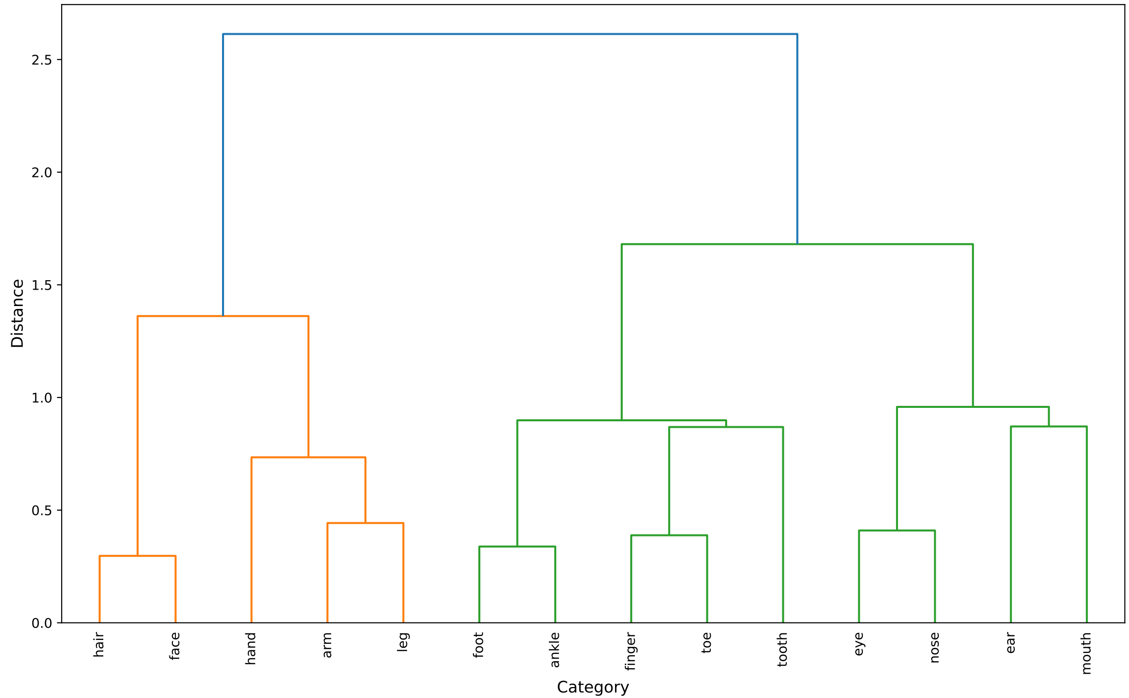
Hierarchical Clustering Dendrogram: BODYPARTS\n(14 categories)
