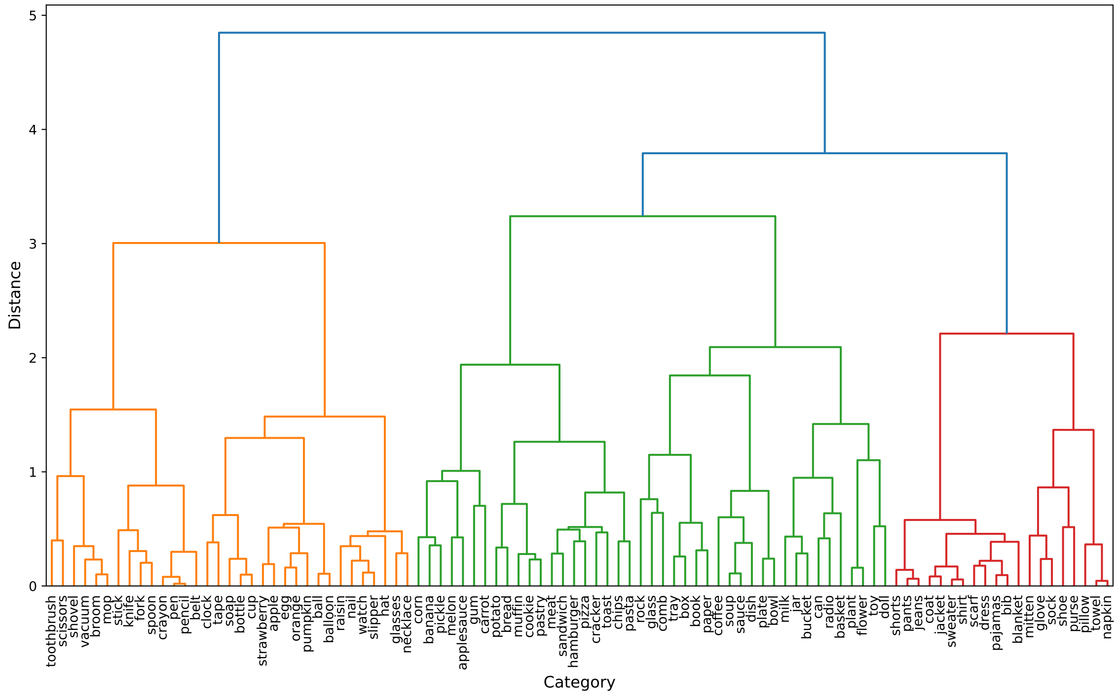
Hierarchical Clustering Dendrogram: SMALL_OBJECTS\n(96 categories)
