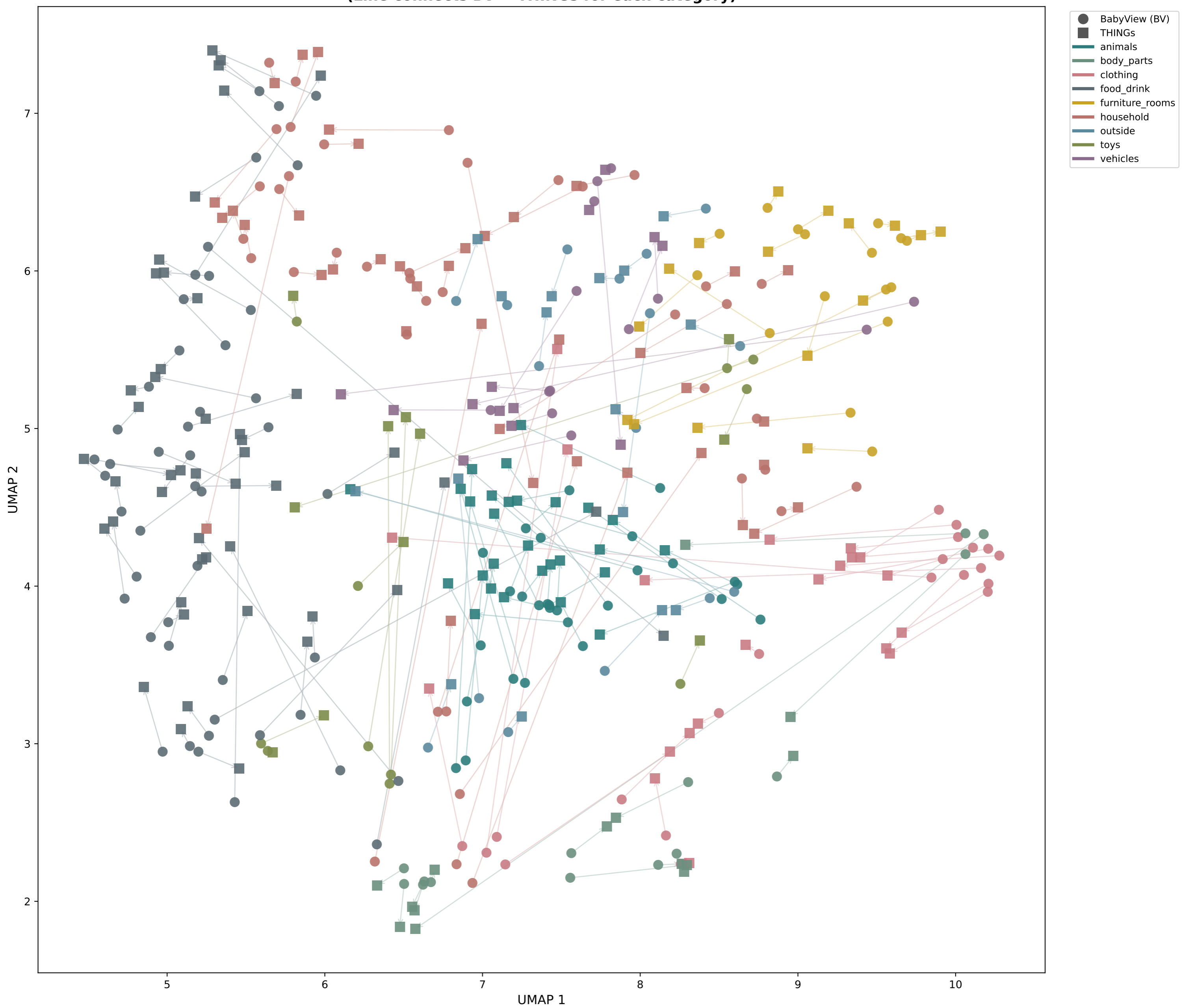
UMAP: BabyView vs THINGS category embeddings (Line connects BV → THINGS for each category)
