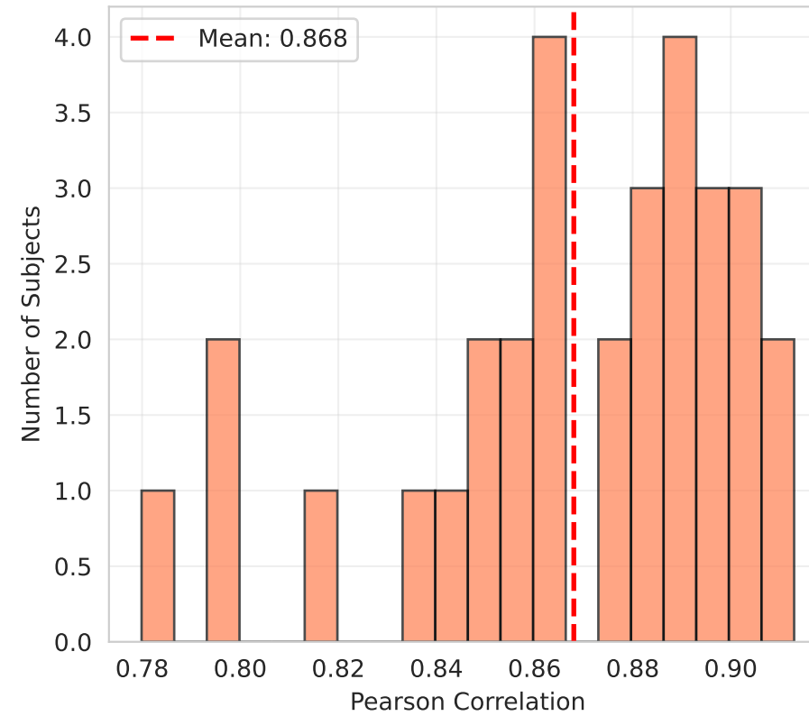
Correlation Comparison
