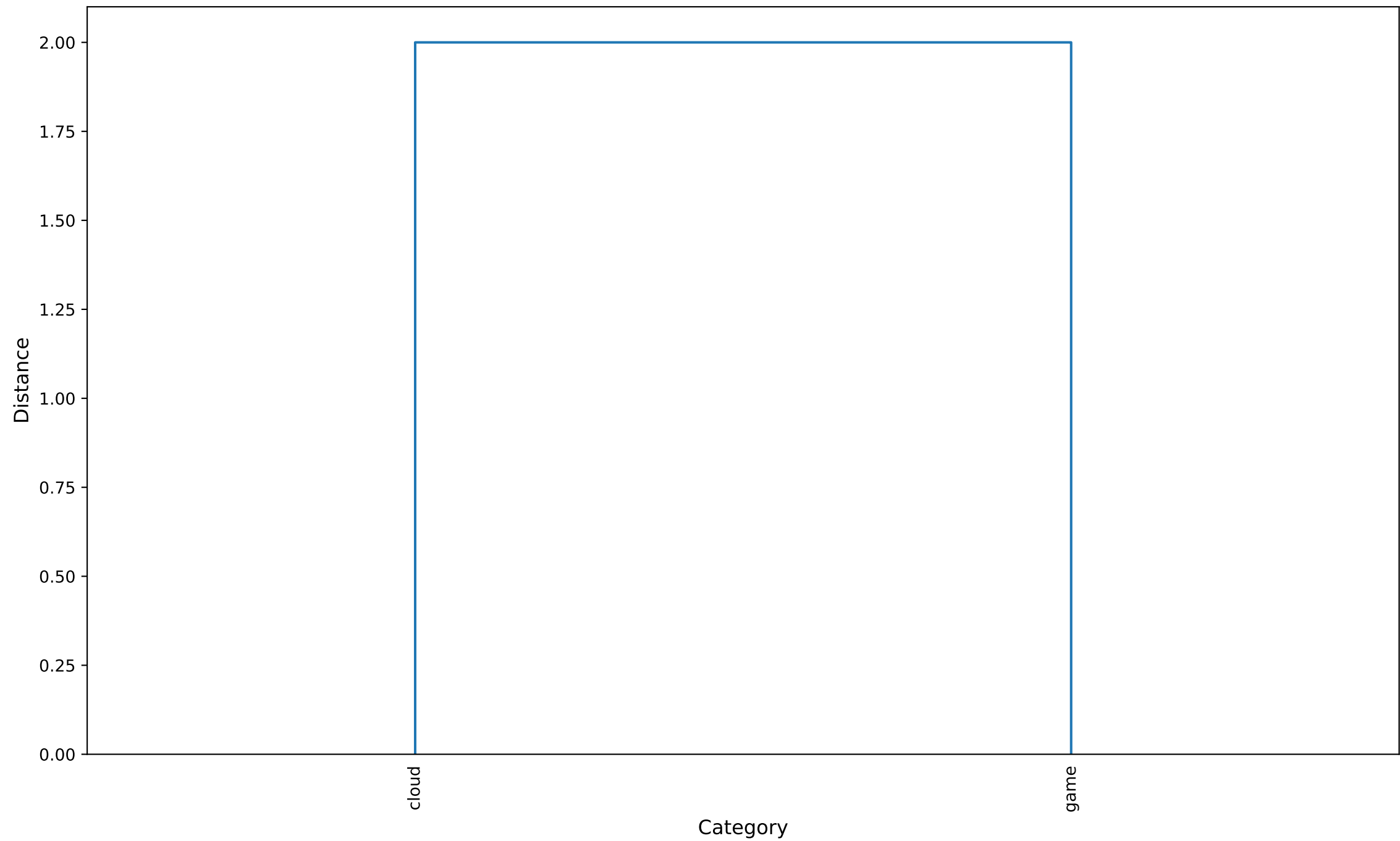
Hierarchical Clustering Dendrogram: OTHERS (2 categories)
