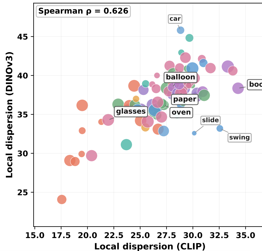
Cross-model local dispersion
