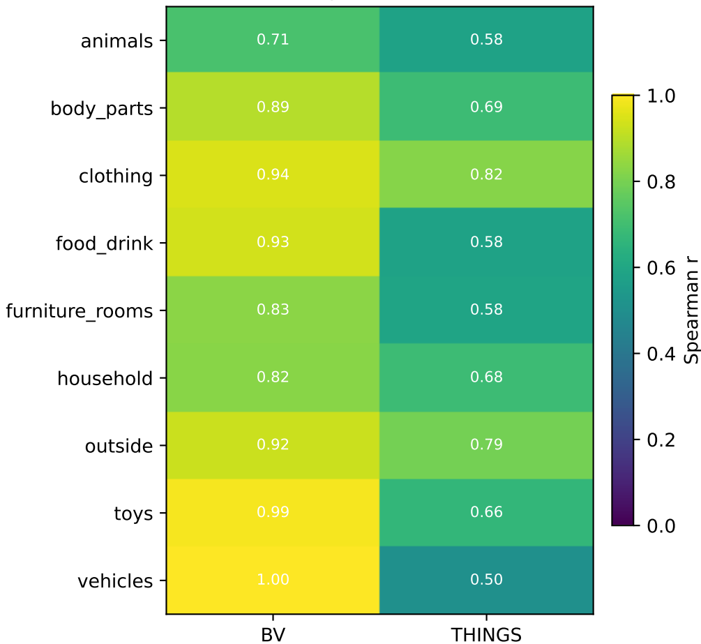
Cluster correlation heatmap (Spearman r)
