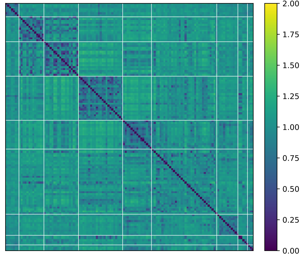
BV RDM (DINOv3, CDI-clustered)
