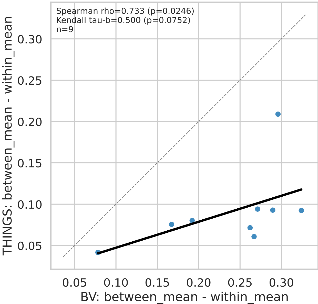
Paired CDI cluster deltas: BV vs THINGS (DINOv3, valid129)
