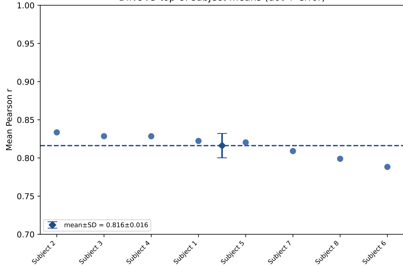
DINOv3 top-8: subject means (dot + error)
