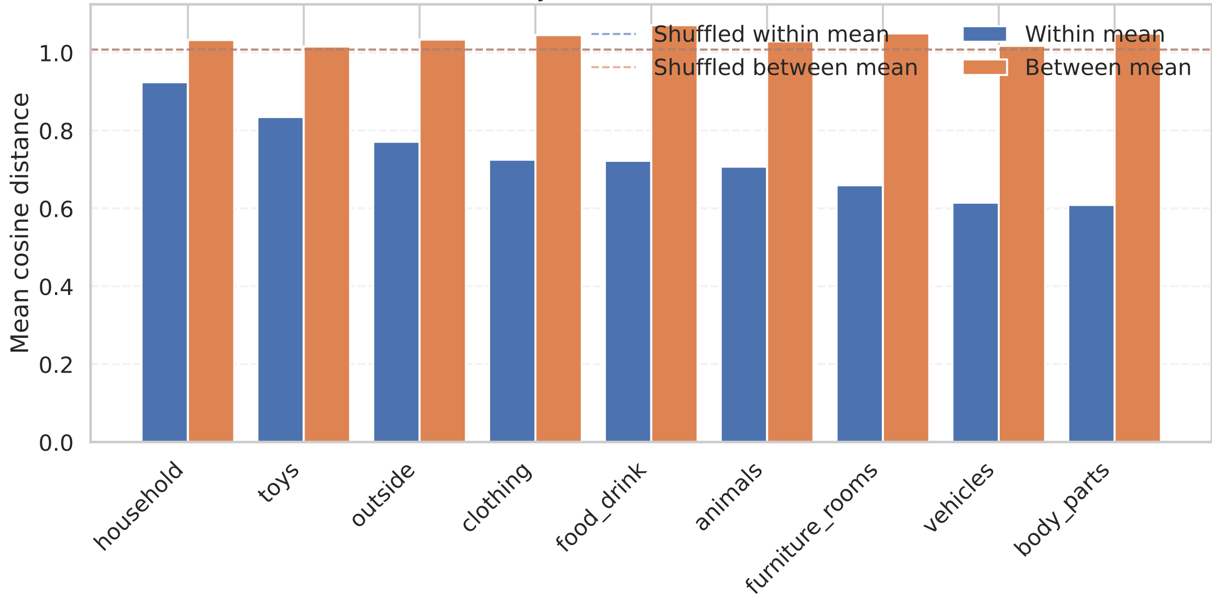
Within vs Between by CDI Semantic Cluster (CLIP, valid129)
