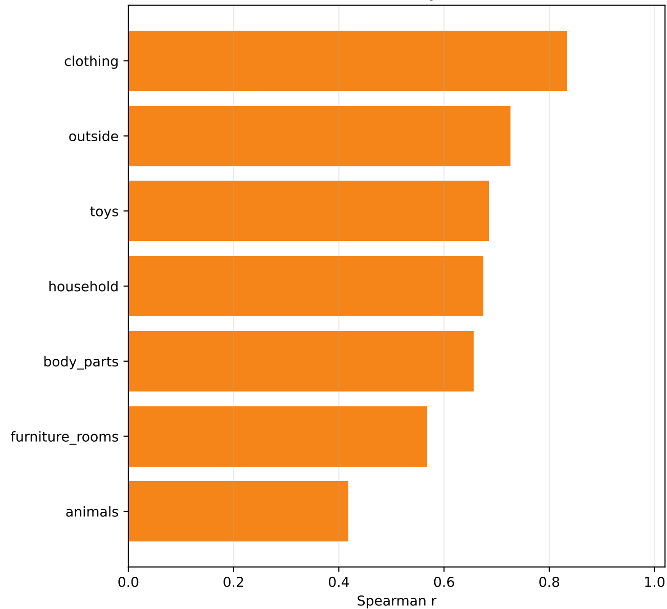
THINGS: CLIP vs DINOv3 by semantic cluster
