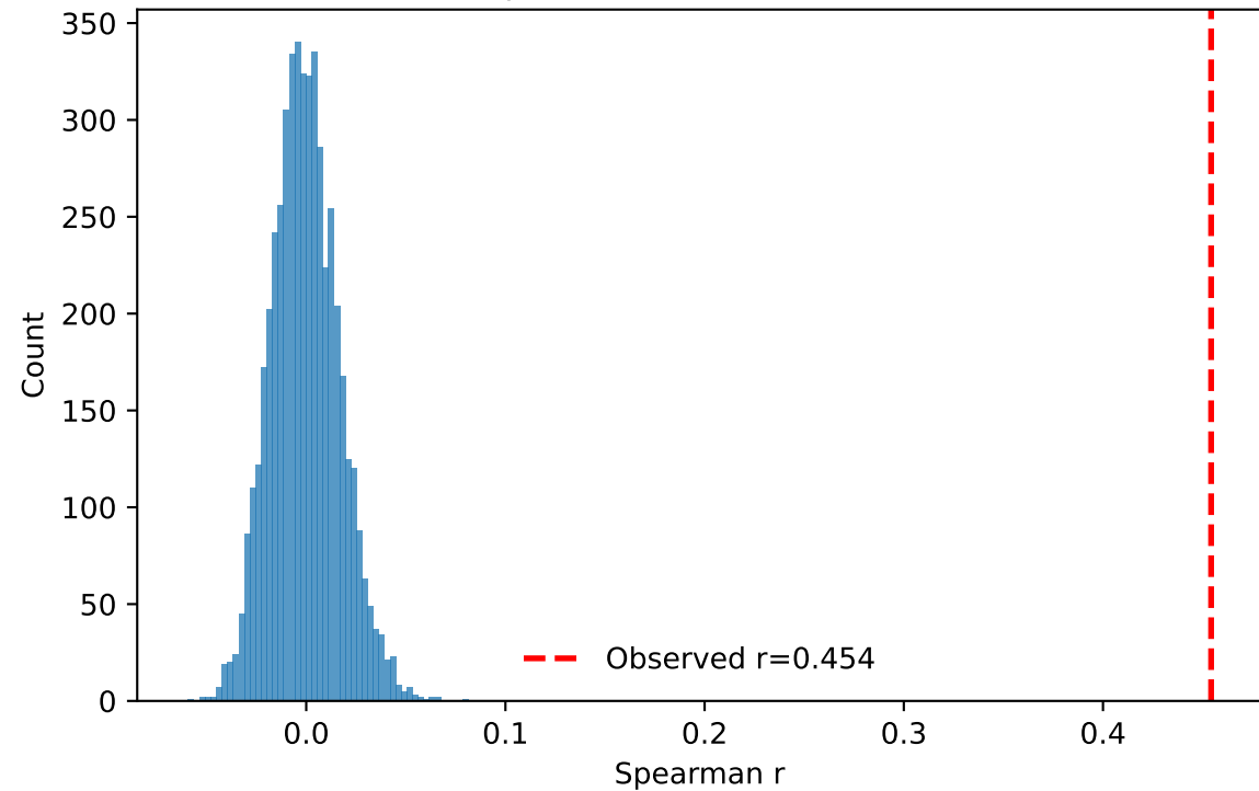
DINO V3 | Independent category shuffle
