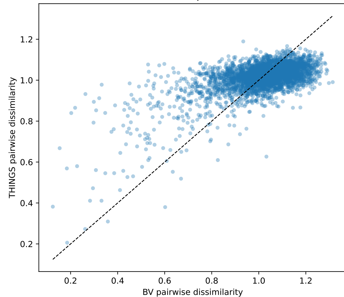
Upper-triangle comparison Pearson=0.624, Spearman=0.454
