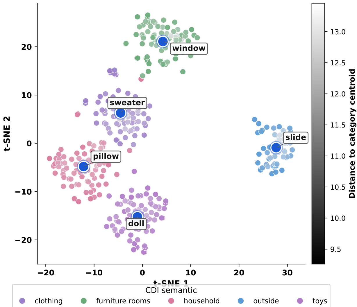
DINOv3 t-SNE (valid7018; one category per CDI semantic group)
