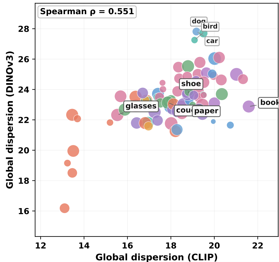
Cross-model global dispersion
