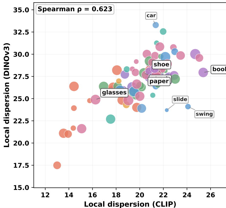
Cross-model local dispersion
