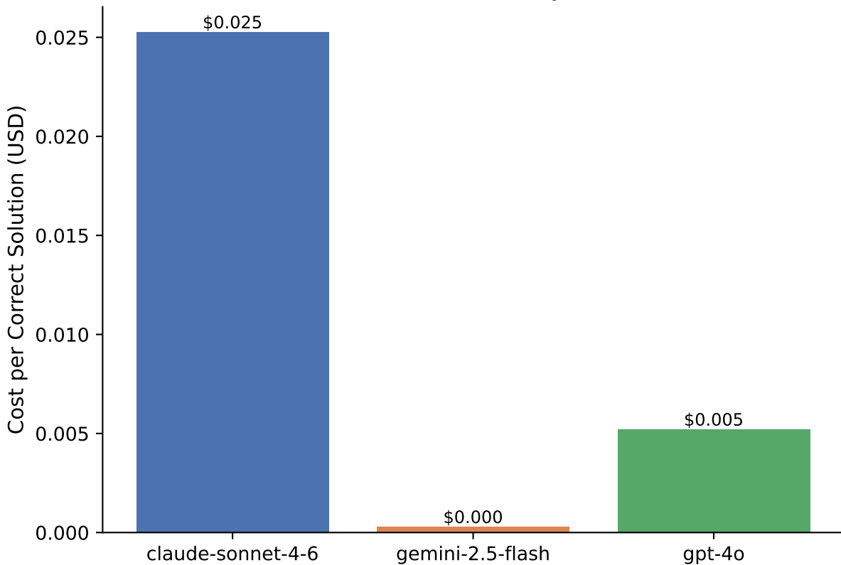
Cost-Effectiveness by Model
