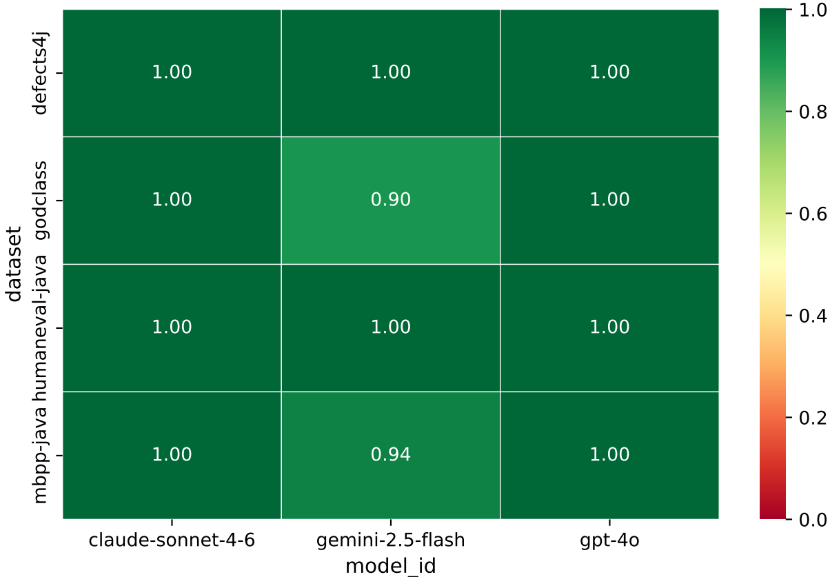
Pass Rate: Dataset × Model
