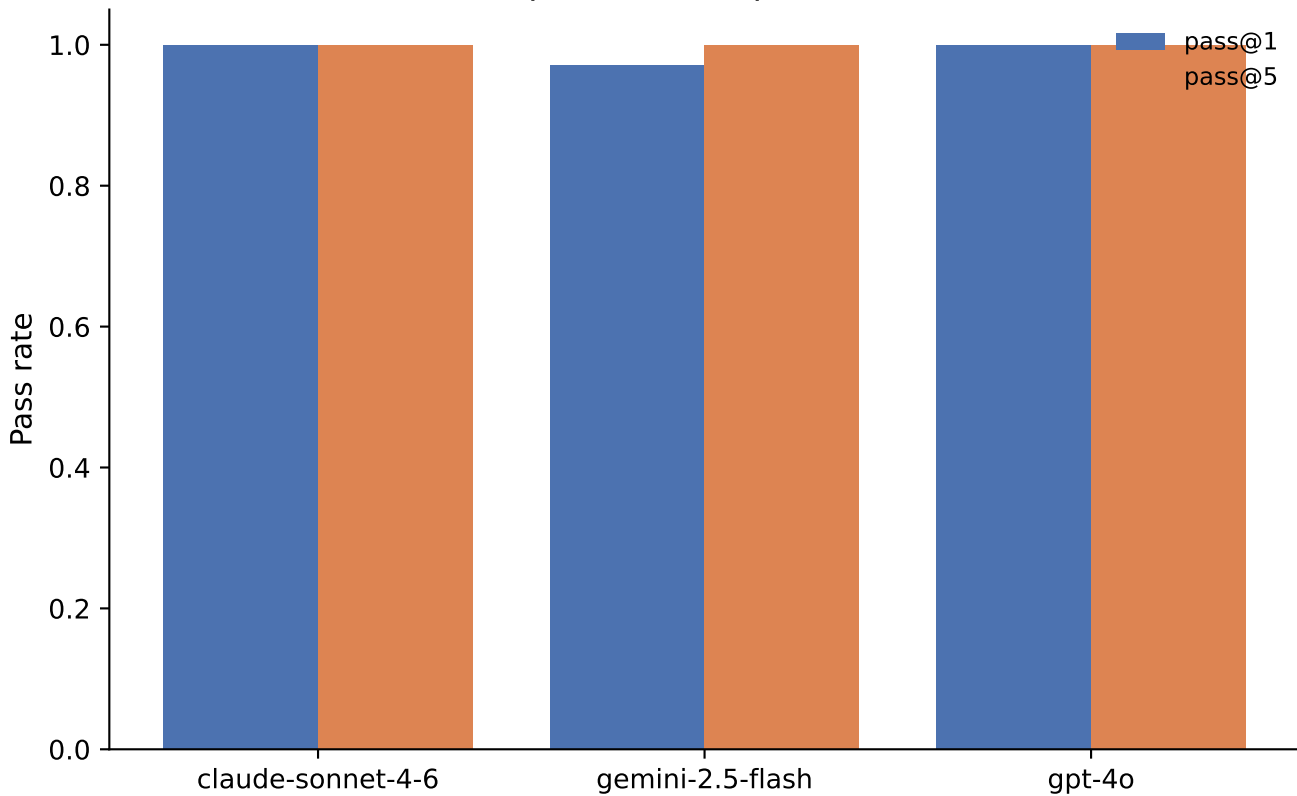
pass@k Comparison
