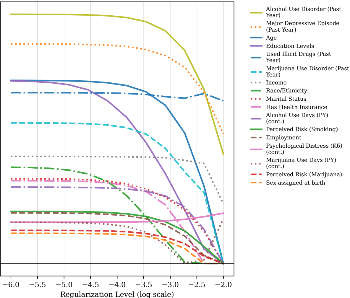
Group-normalized L2 norm of coefficients
