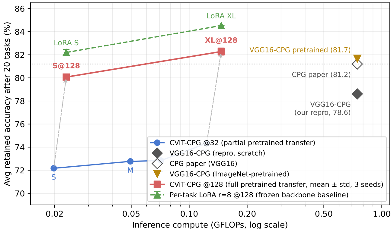
Continual learning accuracy vs inference compute (20-task CIFAR-100; @128 CPG/LoRA points are bit-exact zero forgetting)
