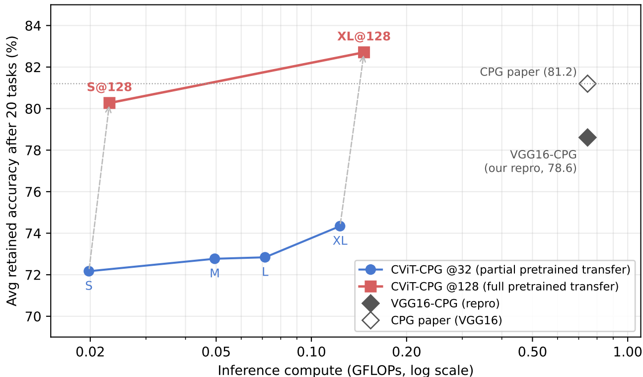
Zero-forgetting continual learning: accuracy vs compute (20-task CIFAR-100, all points bit-exact zero forgetting)
