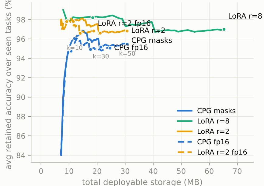
B. Accuracy per storage budget (curves traced by k)
