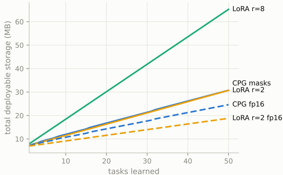
A. Storage growth over the task sequence
