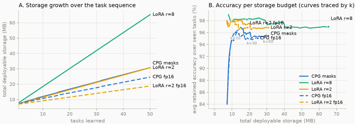
Figure — Same 50-task curve with fp16 per-task stores applied to both mechanisms (Section 9.9).
