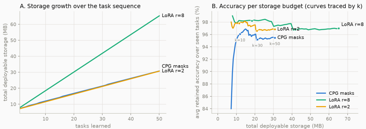
Figure — Cumulative accuracy vs. storage over the 50-task sequence: CPG masks vs LoRA r=2/r=8 , fp32 stores (Section 9.8).
