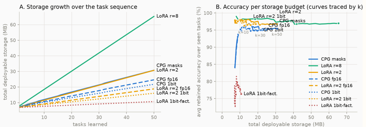
Figure — 1-bit (BitDelta-style) floor compression, both arms; dotted lines are the 1-bit arms (Section 9.9).
