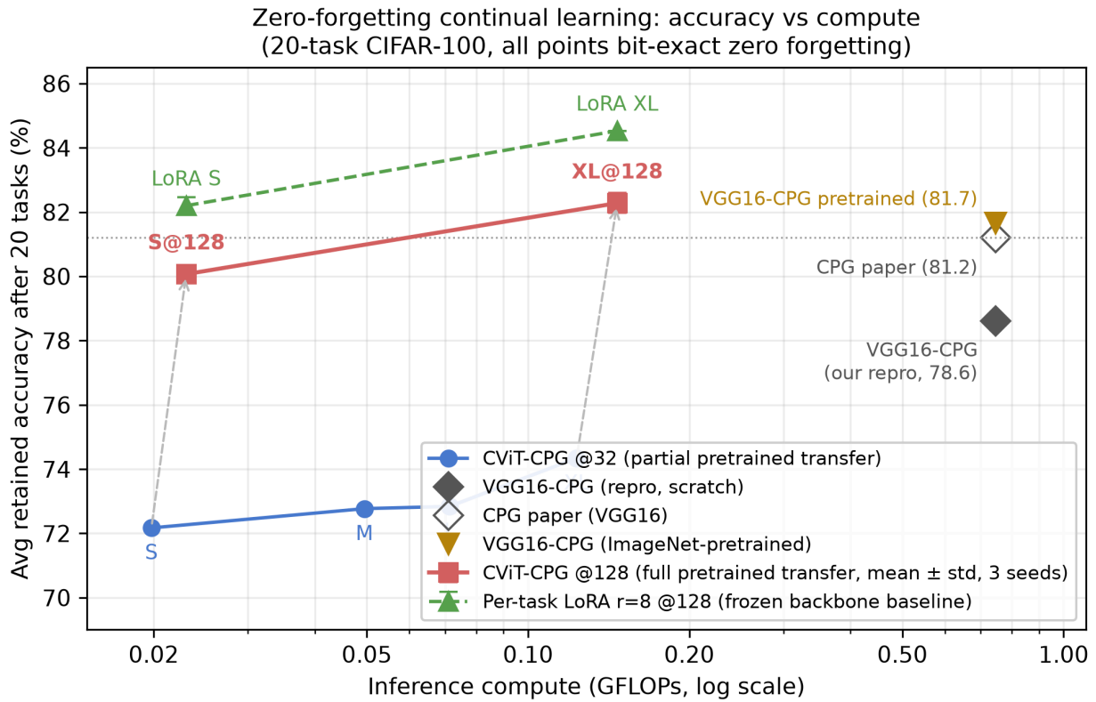
Figure — Accuracy-per-FLOP Pareto frontier: CViT S/M/L/XL vs VGG16-CPG (Section 9.4).
