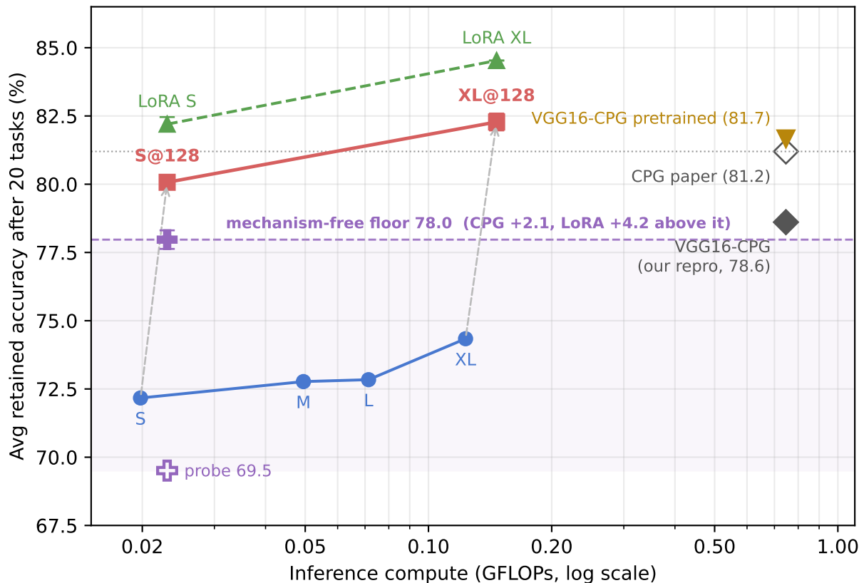
Continual learning accuracy vs inference compute (20-task CIFAR-100; all @128 points are bit-exact zero forgetting)
