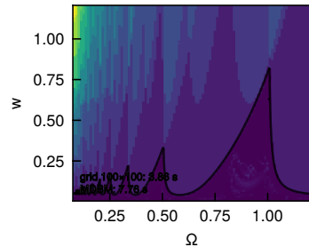
multi-DOF turning lobes
