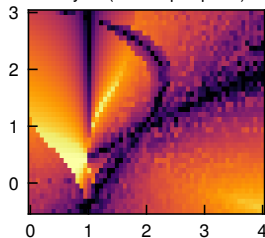
Poly-2 (+3.1% per point)
