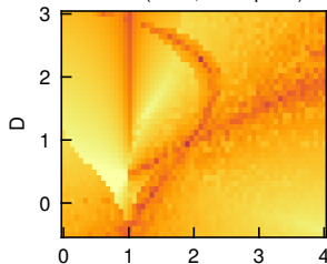
Linear (seed, 2 ms/point)
