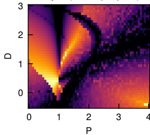
Poly-3 (+9.6% per point)
