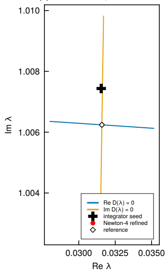
(a) dominant root, zoom \pm 0.0036
