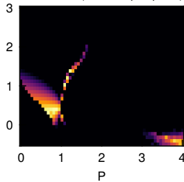
Newton-4 (+10.0% per point)
