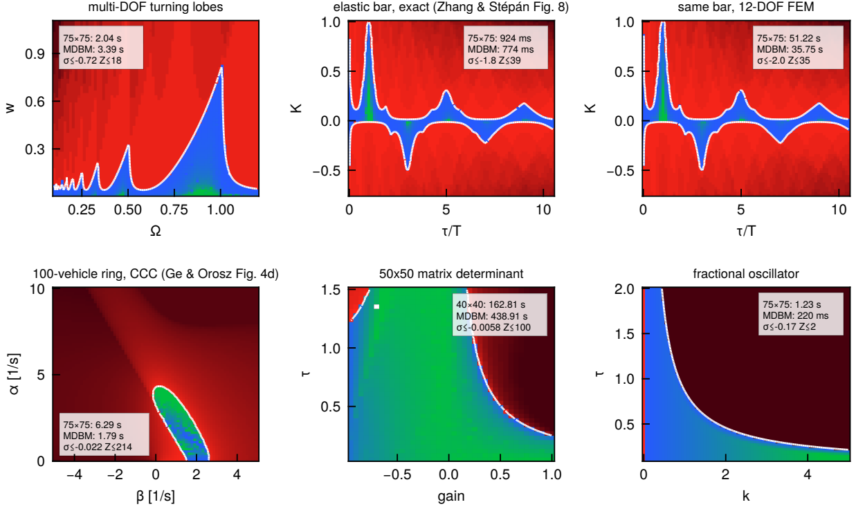
Figure A.11: Case studies, part II: (top row) multi-mode turning lobes, transcendental beam, 12-DOF finite element bar; (bottom row) 50 × 50 matrix determinant, fractional-order oscillator.
