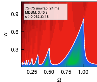
multi-DOF turning lobes
