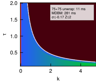
fractional oscillator
