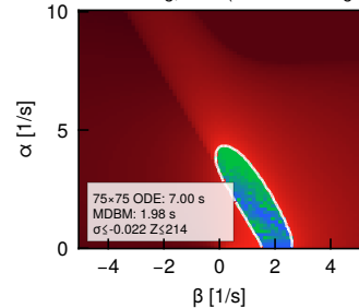
100-vehicle ring, CCC (Ge &amp; Orosz Fig. 4d)
