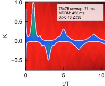
elastic bar, exact (Zhang &amp; Stépán Fig. 8)
