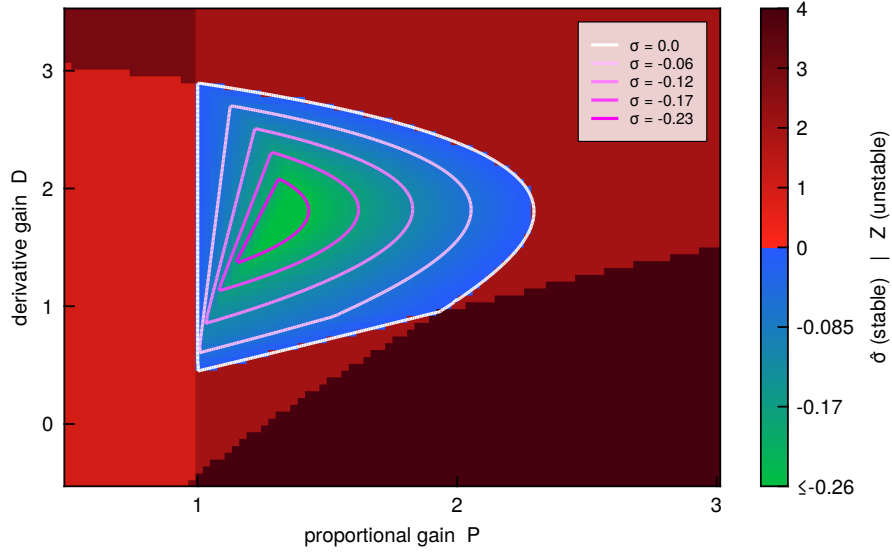
Figure 6: Decay-rate map of the showcase system: colored background – estimated decay rate \hat{\sigma} from the coarse sweep of Fig. 1 (discrete march; stable domain only); curves – \gamma -stability boundaries traced by MDBM for a family of shifted lines \text{Re } \lambda = \sigma . The two independent computations delineate the same landscape.
