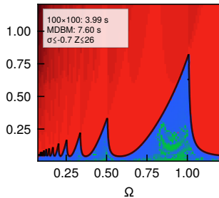
multi-DOF turning lobes
