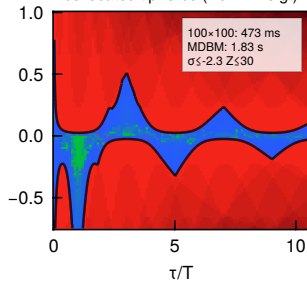
collocated tip force (Kelvin-Voigt)
