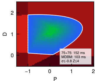
4th-order + delayed PD
