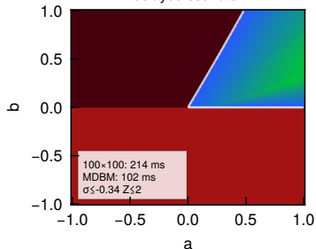
delayed oscillator
