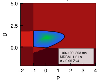
4th-order + delayed PD
