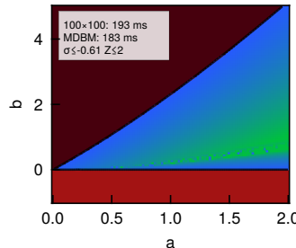
distributed delay
