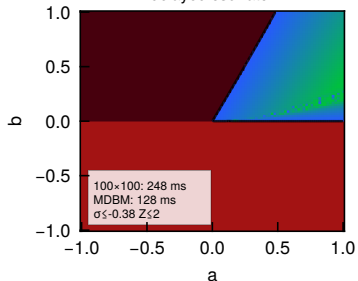
delayed oscillator
