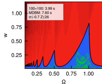
multi-DOF turning lobes
