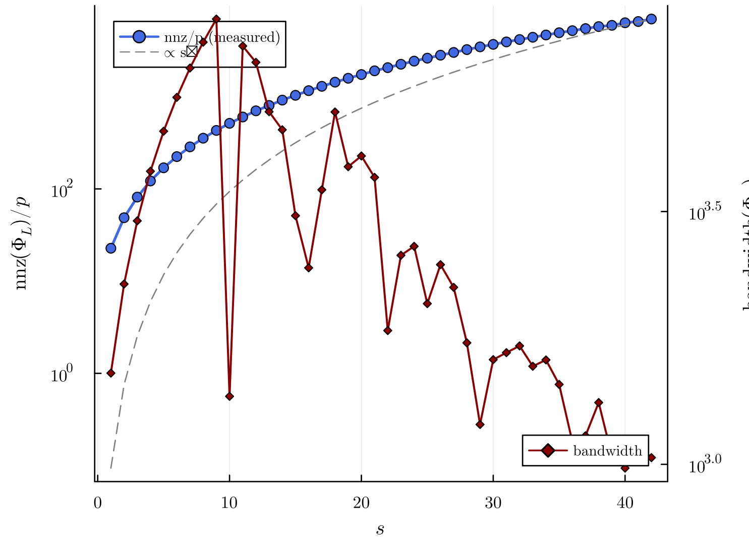
Fill growth — turning_ssv
