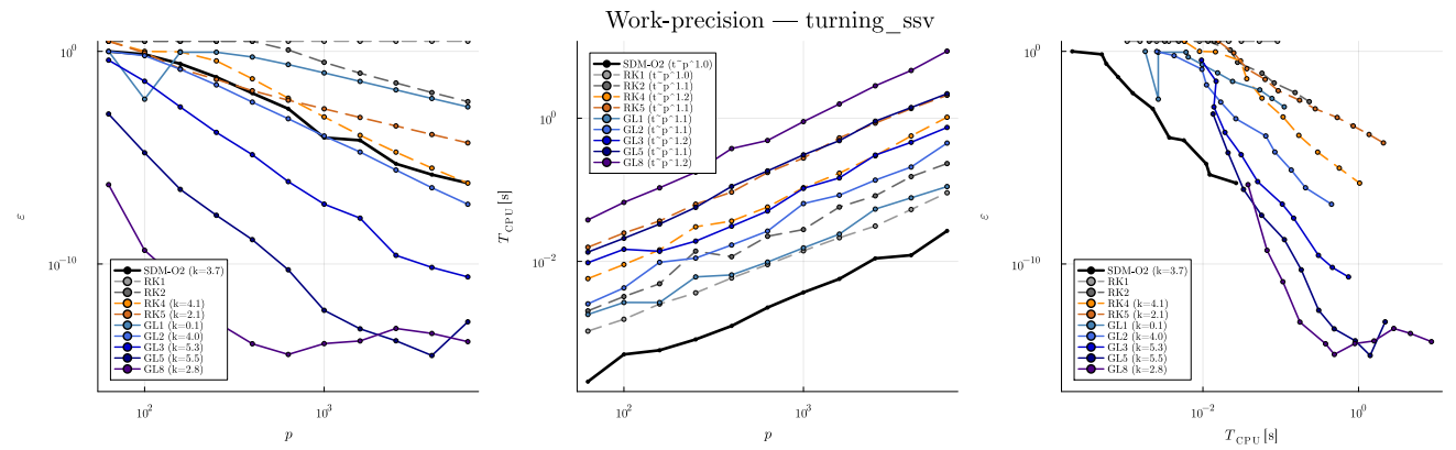
Figure 9. Work-precision study for the turning system with spindle-speed variation; same panel logic as Figure 3, parameters in Appendix .
