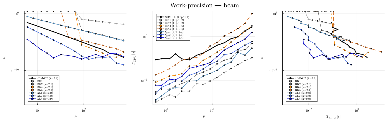
Figure 10. Work-precision study for the FEM beam with delayed boundary feedback. The error axis is clipped at 3 \cdot 10^0 : below the CFL-like stability bound the explicit methods produce meaningless values (up to 10^{43} ), which carry no information beyond “unstable”. CPU times are minima of repeated warm-started benchmark measurements.
