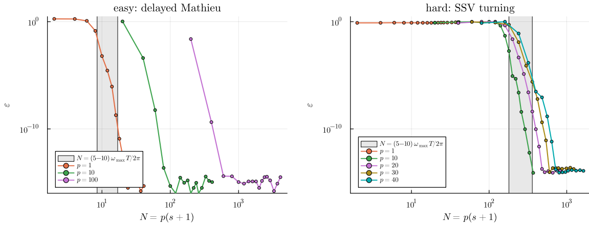
Figure 6. Order refinement at fixed step counts ( p = 1, 10, 100 , left; p = 1, 10, 20, 30, 40 , right): relative error versus the total sample count N = p(s+1) for the easy (left) and hard (right) system, error clipped at 3 \cdot 10^0 . The shaded band is the sampling estimate (10) with c_s = 5-10 . Superconvergent decay starts only once N crosses the band, whose position is set by the oscillation content \omega_{\max} T / 2\pi of the system — not by the method order; on the hard system the single-step curve ( p = 1 ) cannot reach the band within the practical stage range and stays meaningless throughout.
