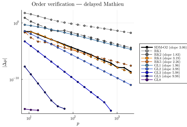
Figure 2. Order verification on the delayed Mathieu equation: eigenvalue error versus resolution p (log–log), one curve per method, fitted slopes in the legend (explicit methods dashed).
