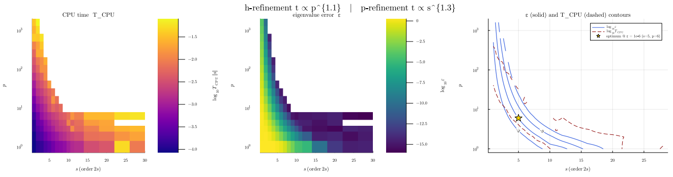
Figure 7. The (s, p) -map for the low-demand delayed Mathieu equation (same three panels as Figure 5): here deep accuracy is reached in the high-order/low- p region as well, and the optima sit near the spectral corner because the matrices stay tiny; the polynomial CPU growth along s is nevertheless visible at the extended stage orders.
