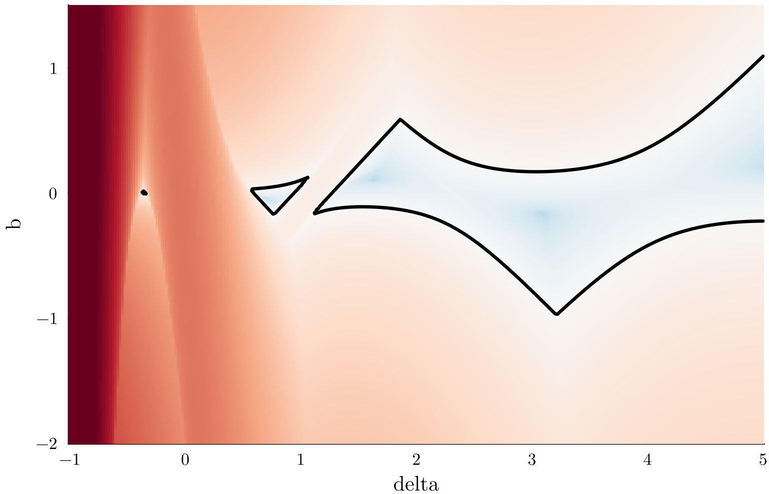
Delayed Mathieu, GL7, p=2 — 122 s (1.3 ms/pt)
