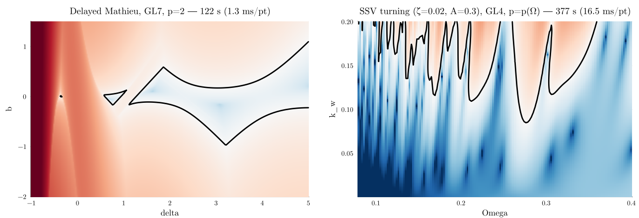
Figure 12. Brute-force stability charts at the optimal settings, coloured by \log_{10} \rho (blue: stable, red: unstable), black curve: stability boundary \rho = 1 ; the measured total CPU time appears in each title. Left: delayed Mathieu equation in the (\delta, b) plane ( \varepsilon = 1 , a_1 = 0.1 , \tau = T = 2\pi ), GL7 with p = 2 . Right: SSV turning in the (\Omega, k_w) plane with strong modulation ( \zeta = 0.02 , A_{SSV} = 0.3 , N_T = 10 ); here the step count follows the sampling recipe of Section per point, p(\Omega) = \lceil 16/\Omega \rceil — the paper's own rule applied in production. All computations single-threaded.
