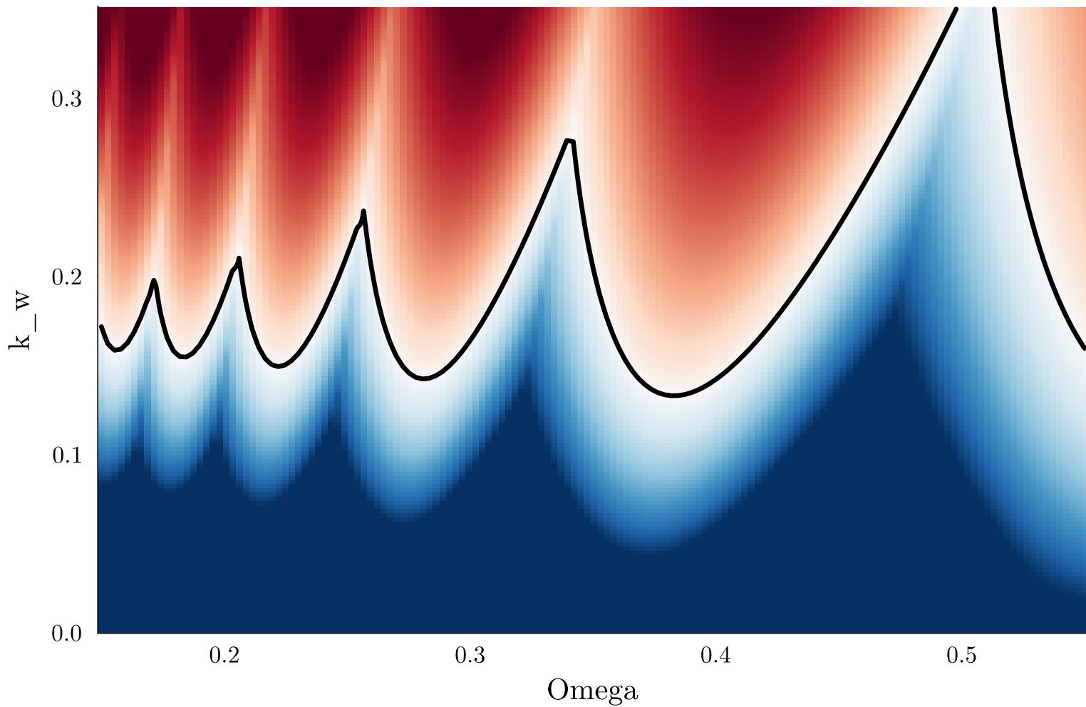
SSV turning — 151x151, GL4, p=158
