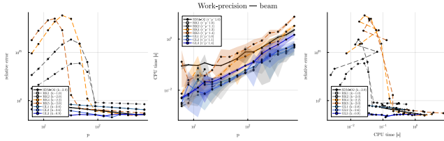
Figure 10. Work-precision — FEM beam with delayed boundary feedback.
