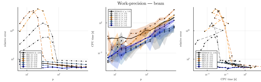
Figure 10. Work-precision — FEM beam with delayed boundary feedback.
