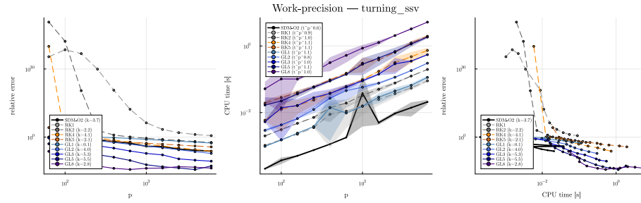
Figure 9. Work-precision — turning with spindle-speed variation.
