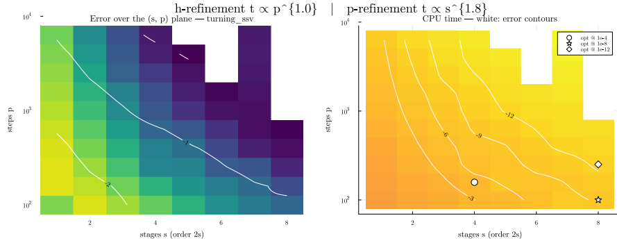
Figure 5. The (s, p) -map for the high-resolution-demand turning system: relative error (left, with white CPU-time contours) and CPU time (right, with white error contours and per-target optima). h -refinement (vertical) is linear in cost, p -refinement (horizontal) polynomial; blank cells exceed the CPU budget. The corresponding maps for the low-demand Mathieu system are in Appendix .
