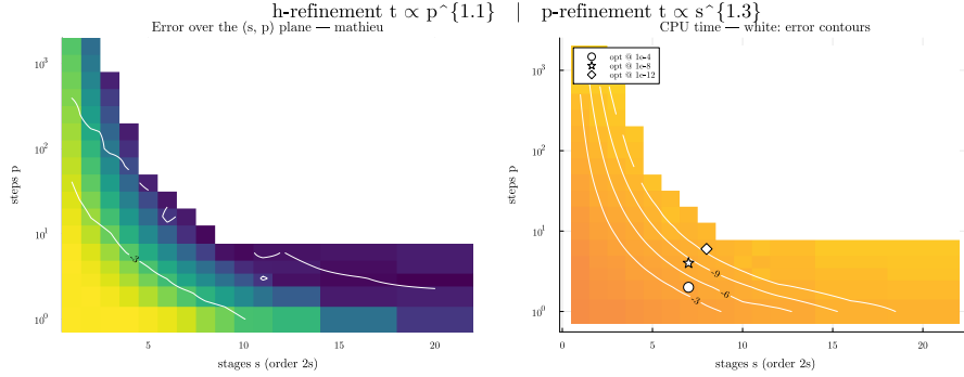
Figure 7. The (s, p) -map for the low-demand delayed Mathieu equation (compare Figure 5): here deep accuracy is reached in the high-order/low- p region as well, and the optima sit near the spectral corner because the matrices stay tiny.
