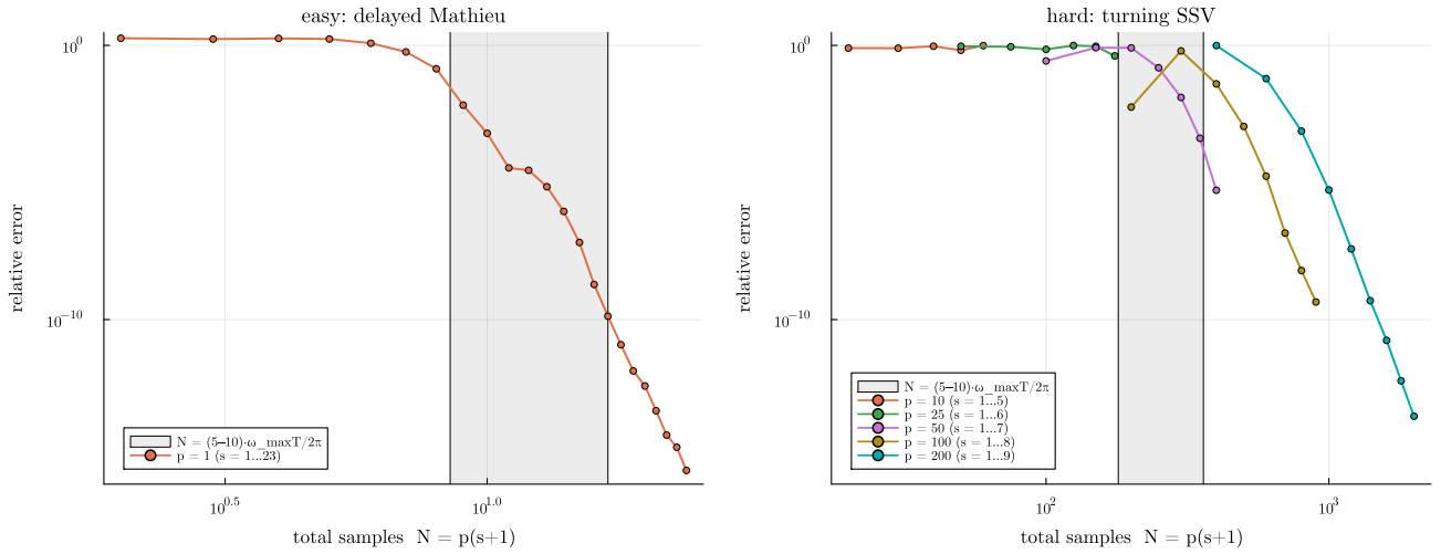
Figure 6. p -refinement at fixed step counts: relative error versus total sample count N = p(s+1) for the easy (left) and hard (right) system. The shaded band is the sampling estimate (10) with c = 5-10 . Super-convergent decay starts only beyond the band; its position scales with \omega_{\max} T / 2\pi , not with the method order.
