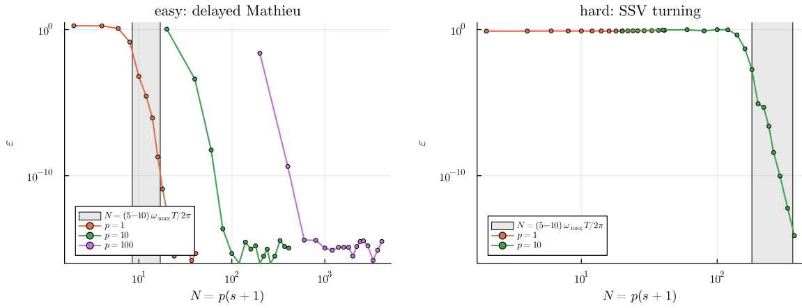
Figure 6. Order refinement at fixed step counts p = 1, 10, 100 : relative error versus the total sample count N = p(s+1) for the easy (left) and hard (right) system, error clipped at 3 \cdot 10^0 . The shaded band is the sampling estimate (10) with c_s = 5-10 . Superconvergent decay starts only once N crosses the band, whose position is set by the oscillation content \omega_{\max}T/2\pi of the system — not by the method order; on the hard system the single-step curve ( p = 1 ) cannot reach the band within the practical stage range and stays meaningless throughout.
