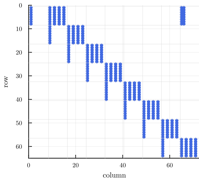
\Phi\_R — Gauss GL3 ( s = 3 ) (nnz = 336)
