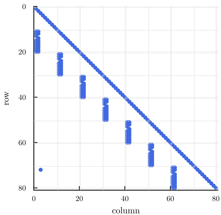
\Phi\_L — explicit RK4 ( s = 4 ) (nnz = 207)
