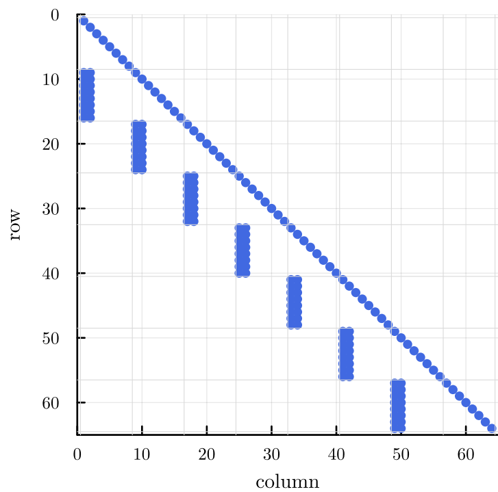
\Phi\_L — Gauss GL3 ( s = 3 ) (nnz = 176)
