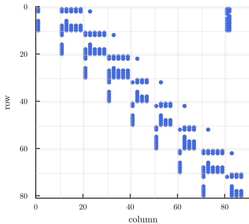
\Phi\_R — explicit RK4 ( s = 4 ) (nnz = 269)
